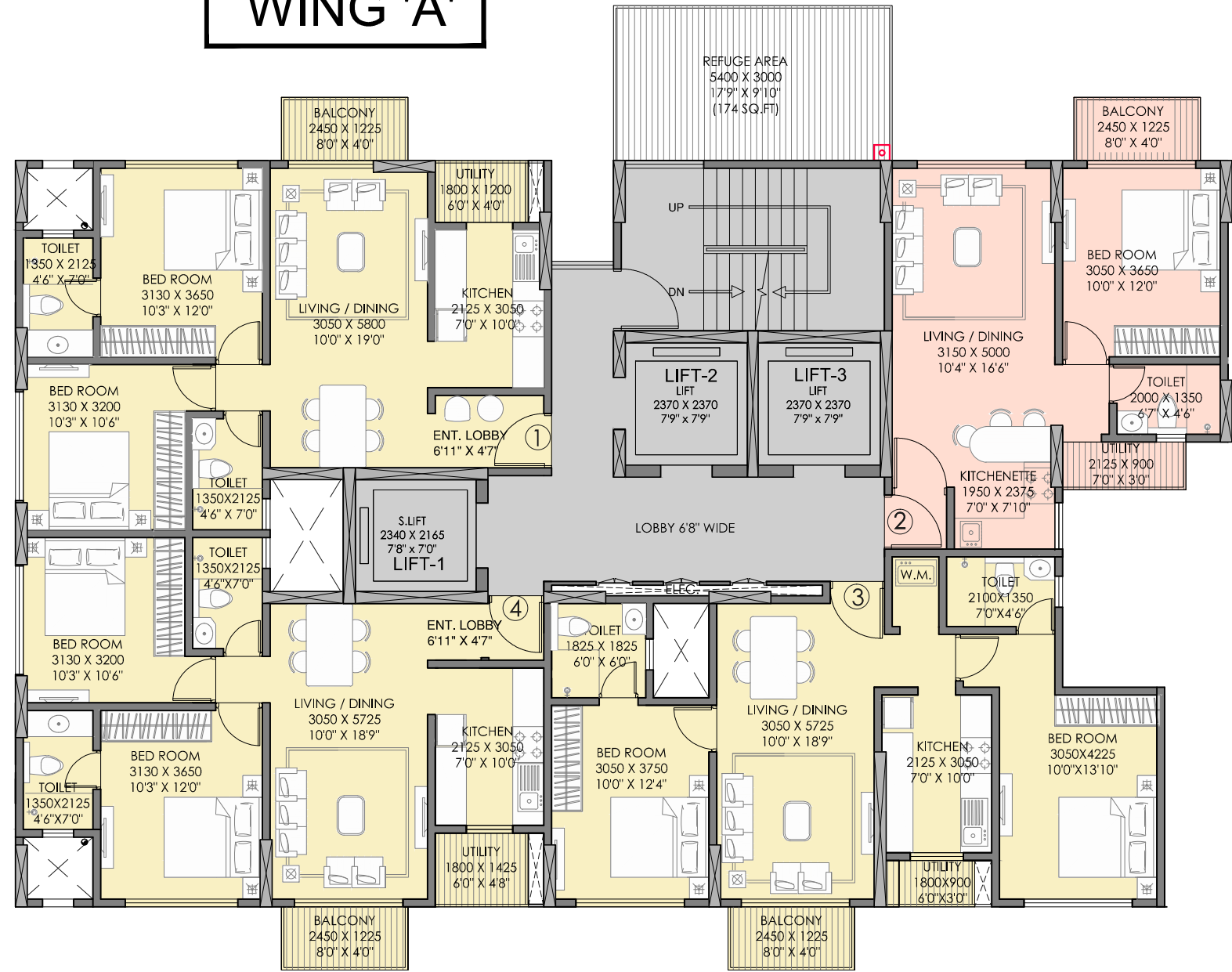
AREA STATEMENT (WING 'A')
